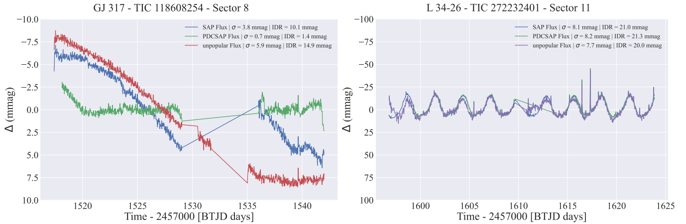
Figure 9. TESS light curves for the two most variable stars in the ATLAS sample: GJ 317 (left) and L 34-26 (right). Light curves are shown from reductions with colors as defined in Figure 4. Note the different y-scale for L 34-26 and the purple color of the unpopular flux which is a result of excluding the polynomial component due to the obvious fast rotation signal that is present in the data.
