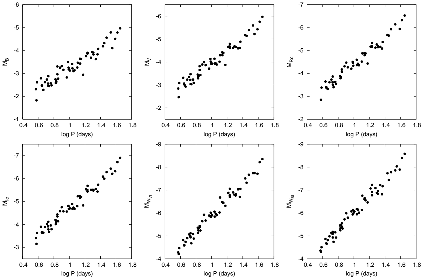
Fig. 2. Adopted Galactic PL relations in optical bands.
