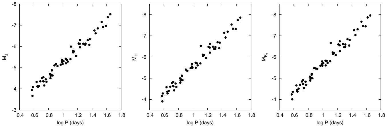
Fig. 3. Adopted Galactic PL relations in near-infrared bands.
